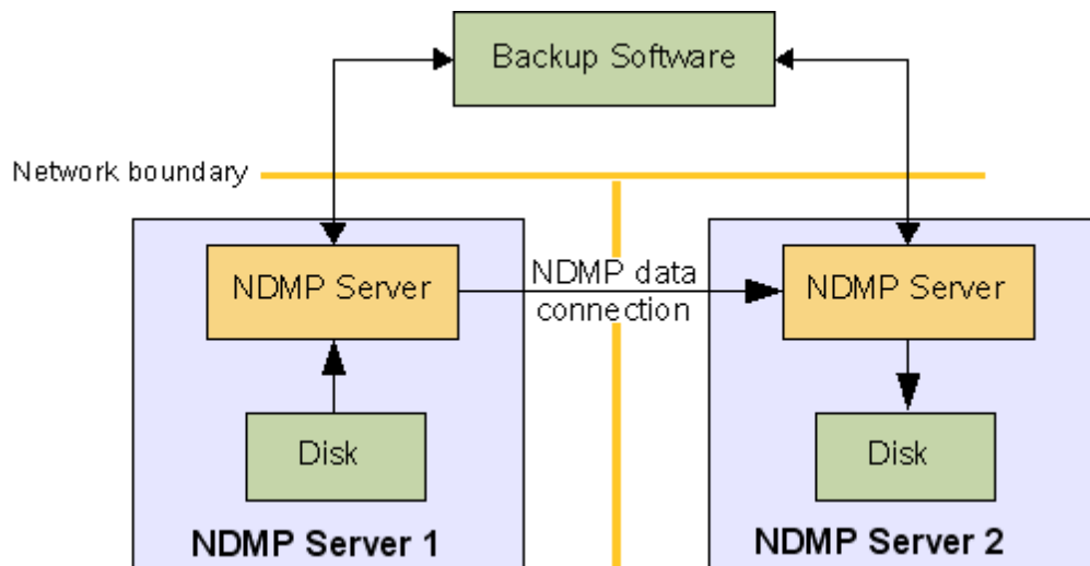
Figure 7 - Disk-to-disk copy
