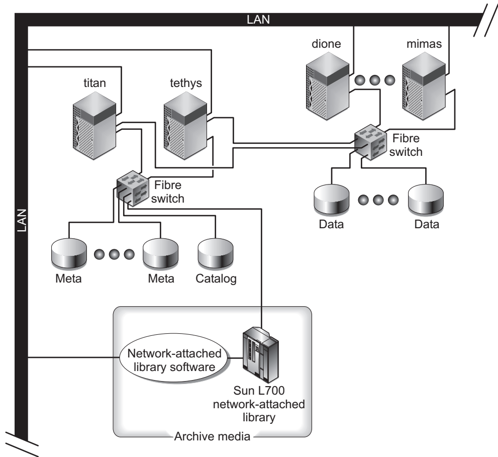
FIGURE D-1 Sun StorageTek QFS Shared File System Configuration in a SAM-QFS Environment
