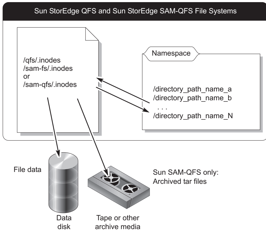
FIGURE 4-1 The .inodes File in Sun StorageTek QFS File Systems
