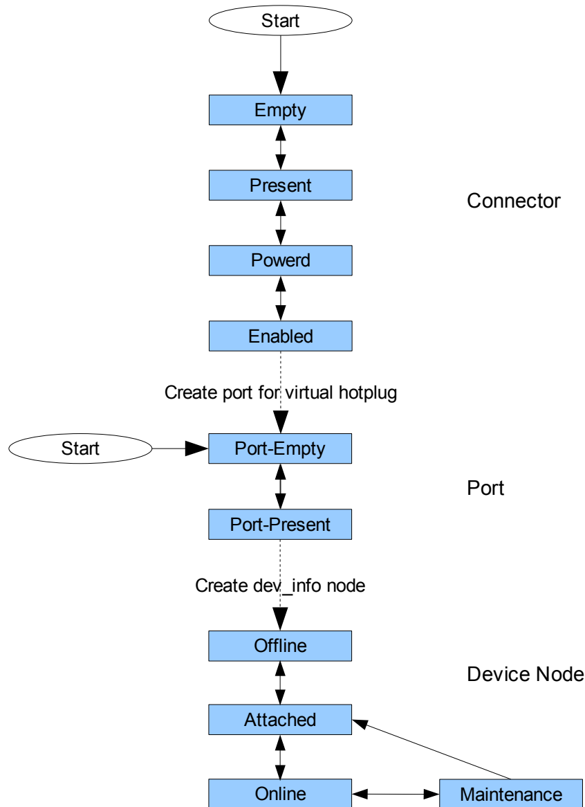
Figure 2. Hotplug State Machine
